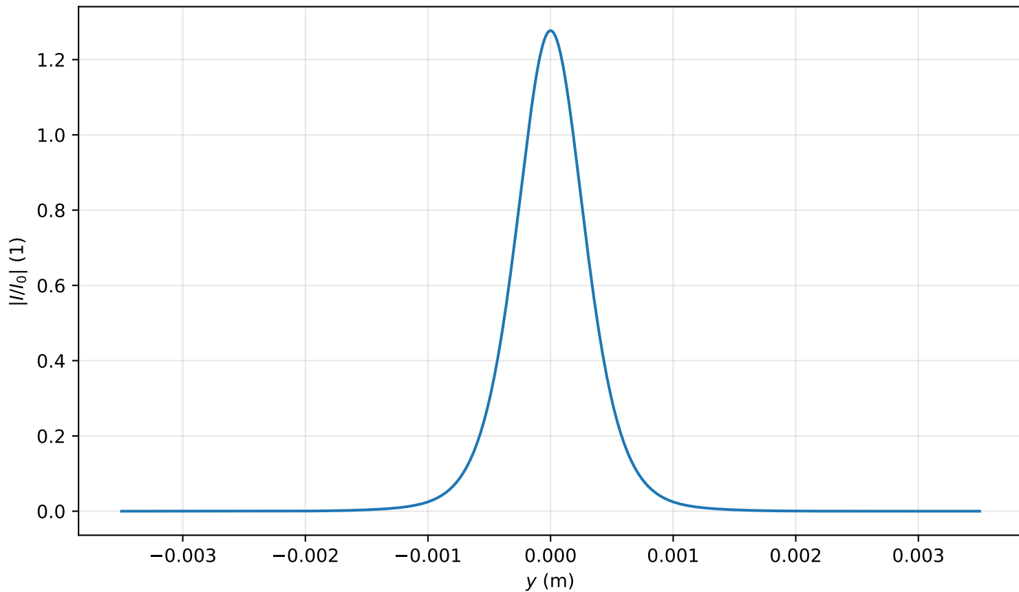
Intensity profile I(x=0, y, z=2.229)/I_0 , P_{in}=0.8P_{cr} , artificial time
